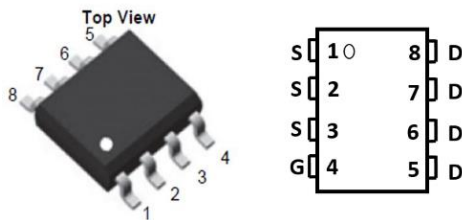
SOP-8 SES8619AG
