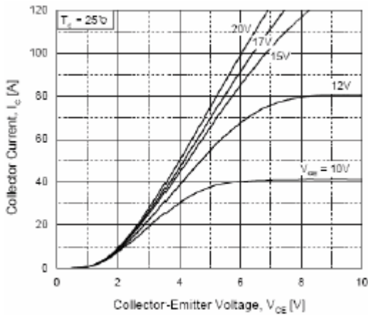
Fig.1 Out Characteristics
