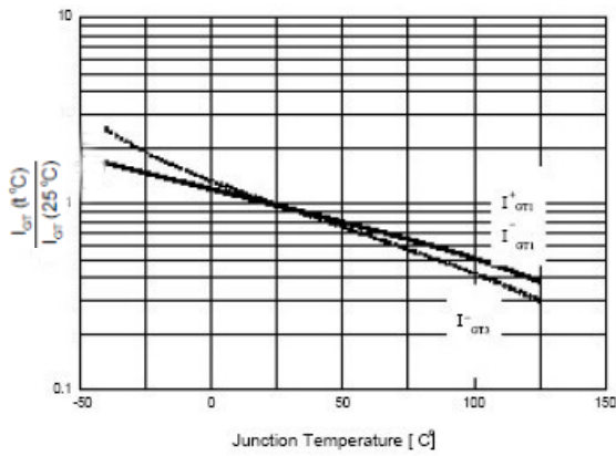
Fig.7 Gate Trigger Current vs. Junction Temperature
