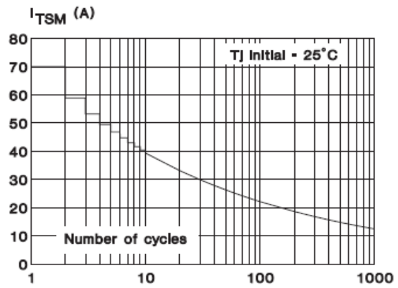
Fig.4 Maximum permissible non -repetitive peak on-state current I_{TSM} , versus number of cycles, for sinusoidal currents. f=60\text{Hz}
