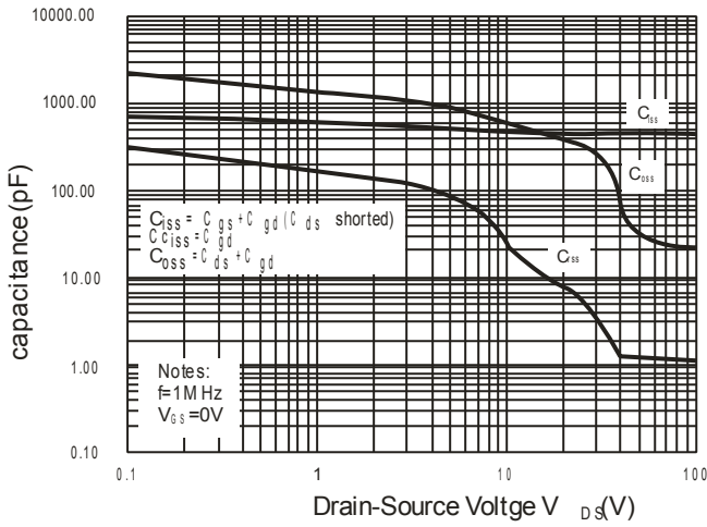
Fig.7 Capacitance Characteristics
